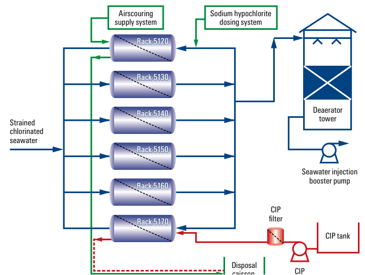
Process flow schematic.
