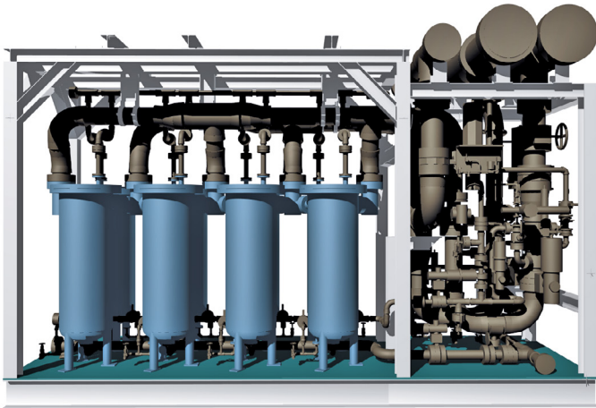
Membrane modules on a single skid.
