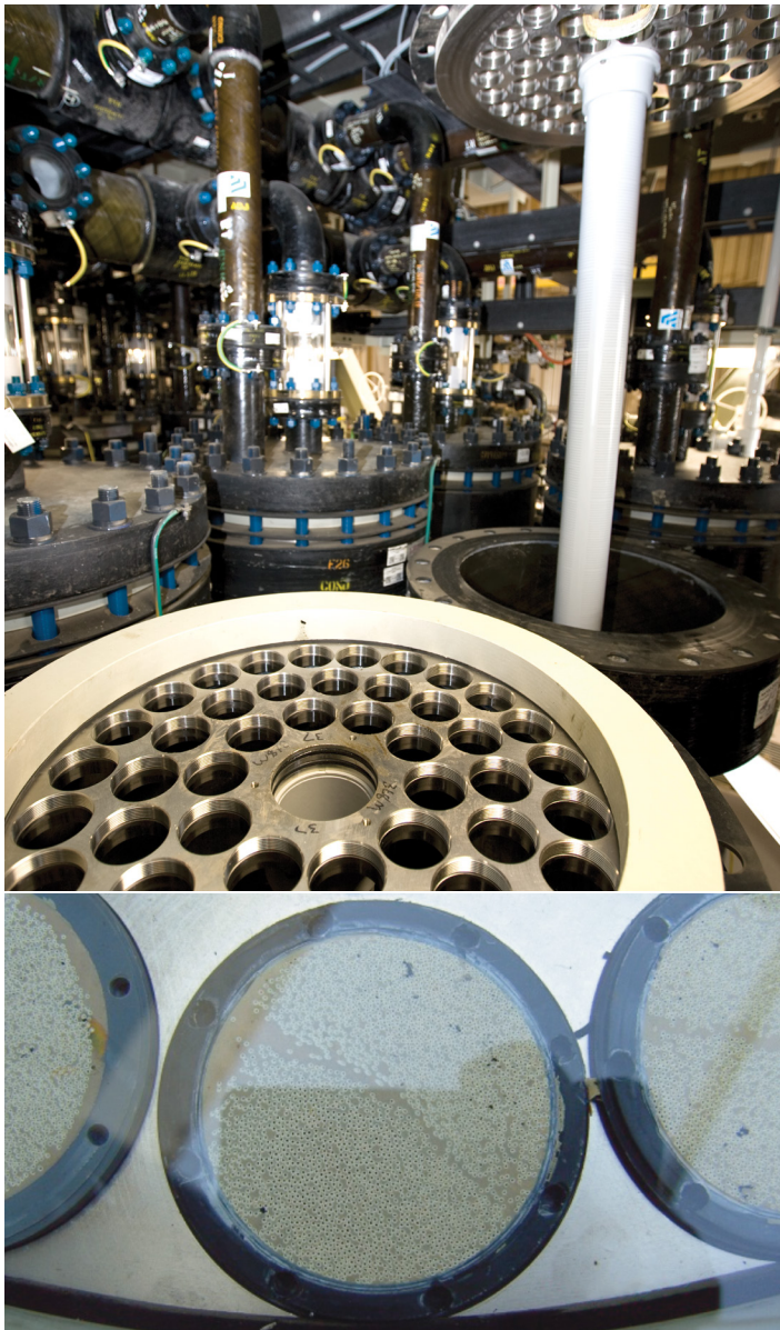
There are 49 bundles contained in a 24-in diameter module. Pictured (bottom) is one bundle filled with hollow membrane fibers.
