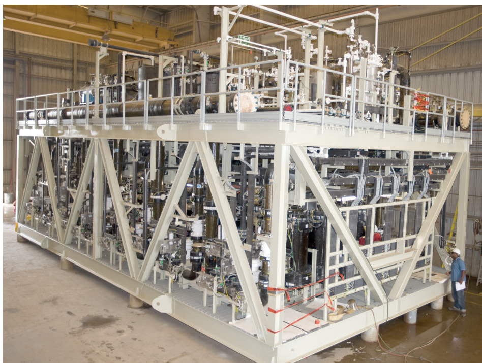
Total Ofon 2 Polymem UF system ready for shipment.
