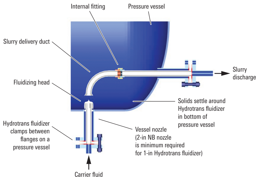
Hydrotrans fluidizer.
